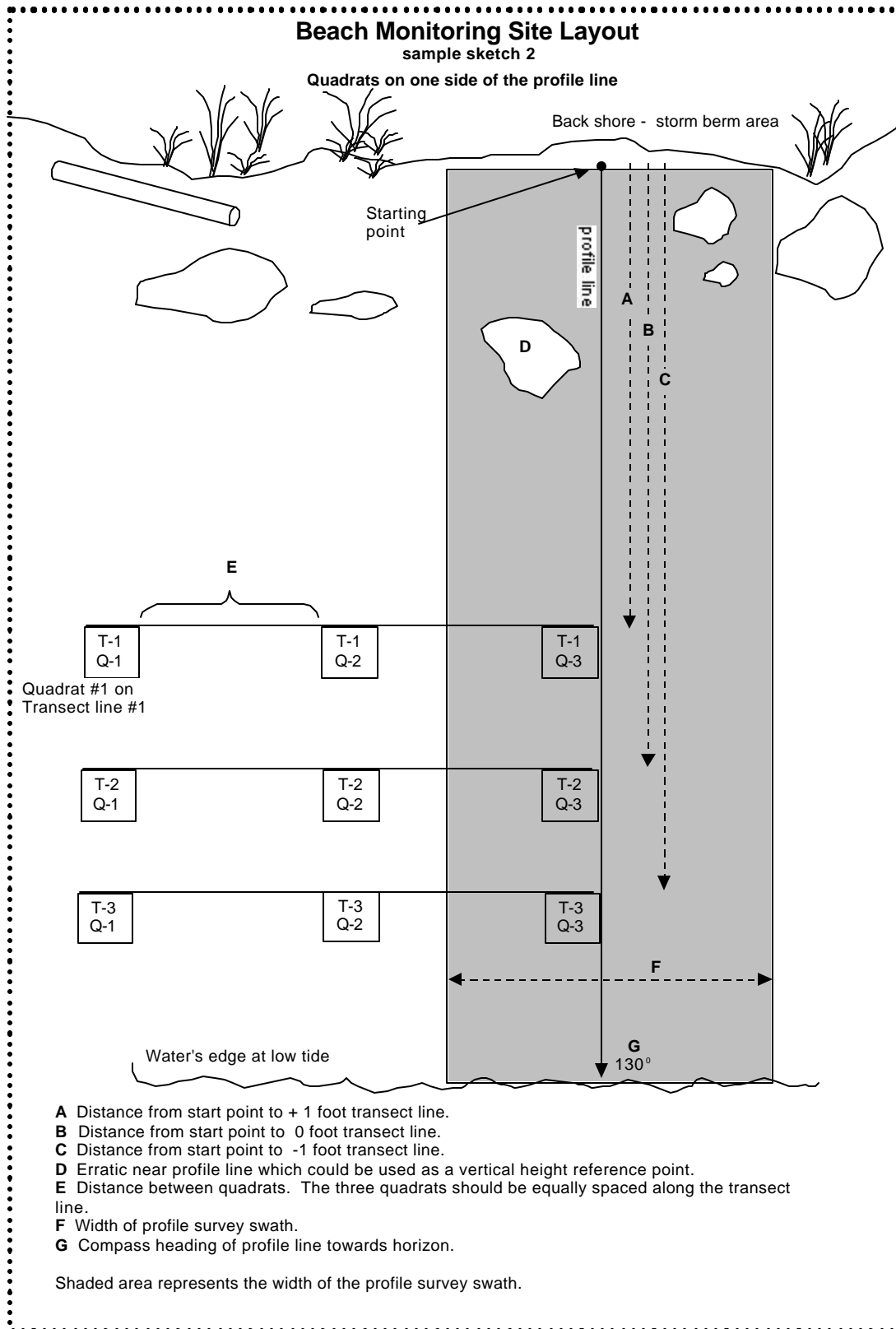
FIGURE 1b. Beach Monitoring Site Layout, Sample #2
