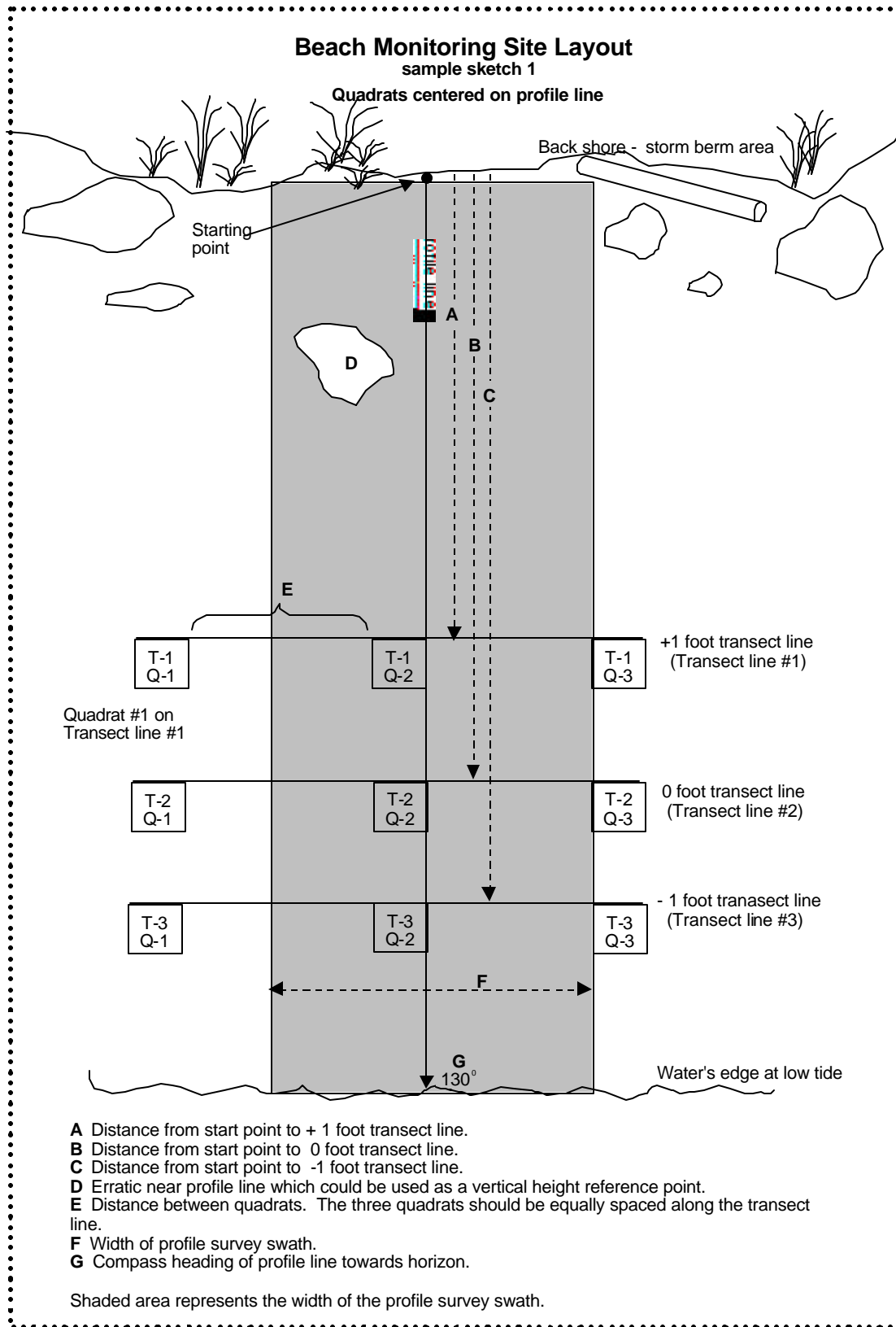
FIGURE 1a. Beach Monitoring Site Layout, Sample #1
